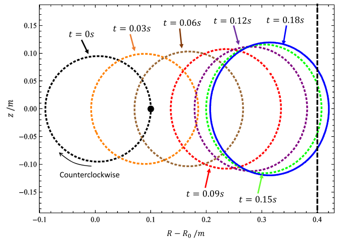
FIG. 3. Snapshots, taken for every 0.03 s, of the circular orbit of a runaway positron in the poloidal plane, with initial position R - R_0 = 0.1 m, z = 0 m and initial momenta p_{||} = 5m_e c and p_{\perp} = m_e c . The loop electric field is E_l = 5 V/m. The position of the first wall is indicated by the dashed vertical line.
