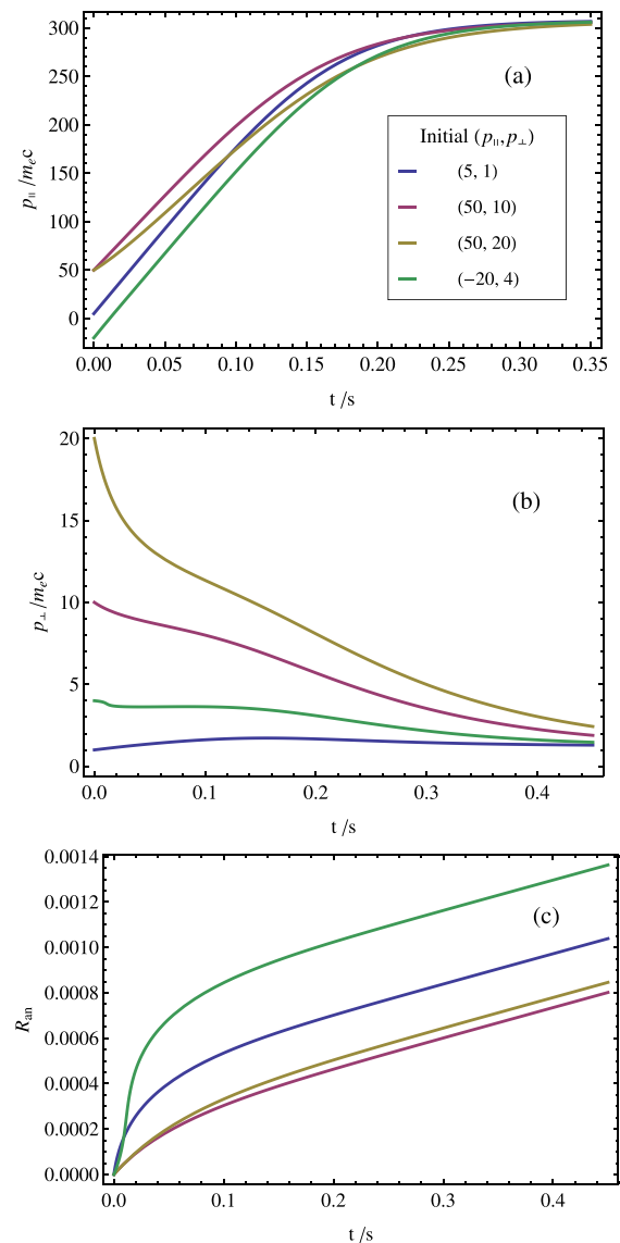
FIG. 2. The evolution of the parallel momentum (a), the perpendicular momentum (b), and the annihilation rate (c) of runaway positrons in tokamaks with different initial values of (p_{\parallel}, p_{\perp}) (normalized by m_e c ). The loop electric field is E_l = 3 V/m.
