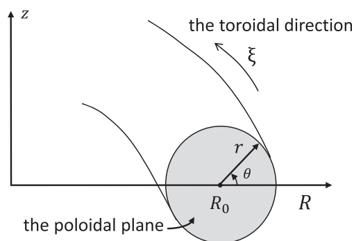
FIG. 1. The circular concentric magnetic flux surfaces and the coordinate systems.
