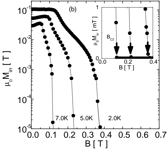
Figure 3: (a) Reversible magnetization of a BCP sample at 2 - 7 K, evaluated from the isothermal loops. (b) Irreversible magnetization at 2, 5 and 7 K, showing the sharp onset of bulk superconductivity at B_{c2}(T) = \mu_0 H_{c2}(T) .
