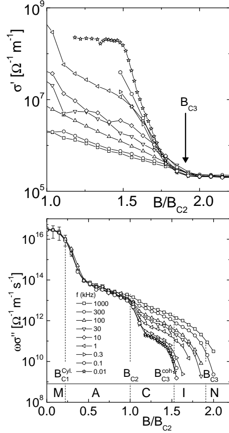
Figure 15: The complex conductivity \sigma(\omega) as a function of field for frequencies between 10 Hz and 1 MHz. The top graph shows \sigma' , the bottom graph \omega\sigma'' . The indicated critical fields B_{c1} , B_{c2} , B_{c3}^{coh} and B_{c3} separate five phases: Meissner M, Abrikosov A, coherent surface superconductivity C, incoherent surface superconductivity I, normal state N.
