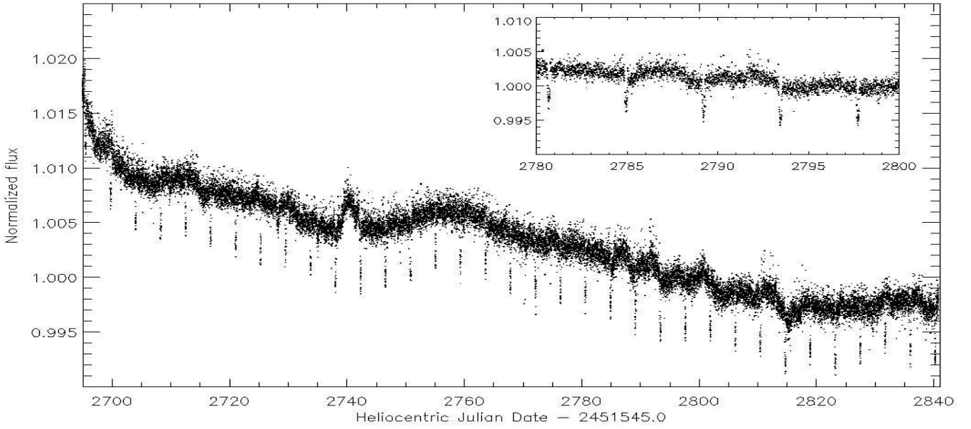
Fig. 1: The 152-days long CoRoT-Exo-3b reduced light curve, binned at a constant time sampling of 512 sec and normalized. The low activity level of the star is illustrated in the upper figure which displays a zoomed section of the light curve.
