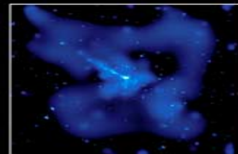
CHANDRA X-RAY
