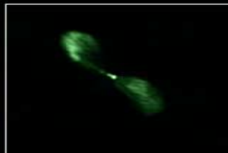
NRAO RADIO CONTINUUM
